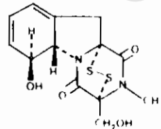
Gliotoxin
