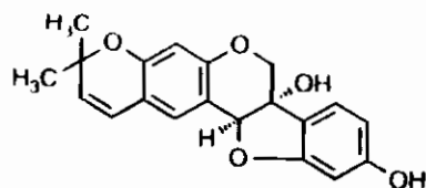
Glyceollin II
