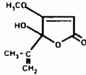
Penicillic acid
