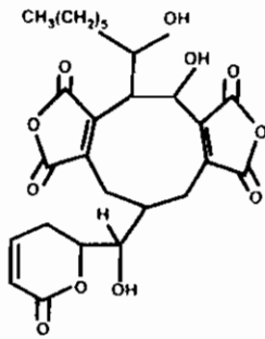
Rubratoxin B
