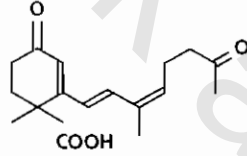
Trisporic acid شكل (٥٨٠)
