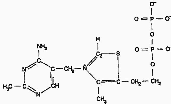
Thiamin pyrophosphate
