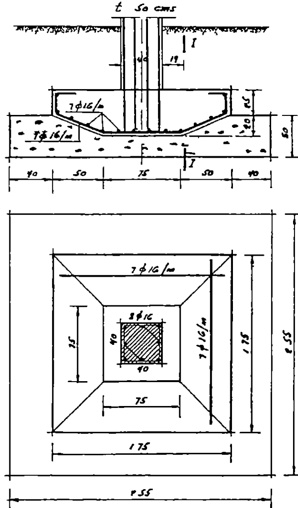
DETAILS OF AN ISOLATED FOOTING
