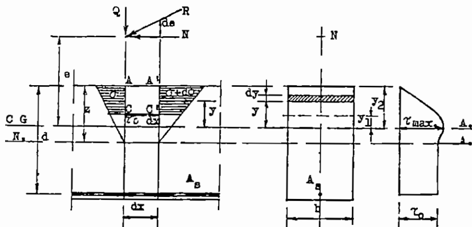
Fig 2-50 Shear stresses in a section subject to eccentric force with big eccentricity
