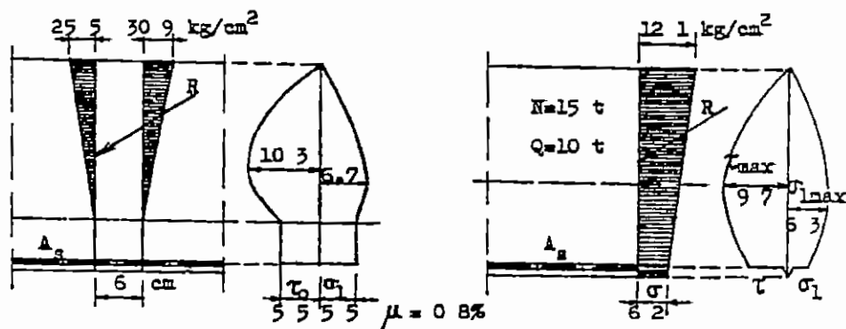
Fig 2-53 Shear and principal tensile stresses in sections subject to eccentric compression with small eccentricity
