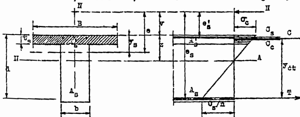
Fig 2-43 Stresses in a T-section subject to eccentric forces with big eccentricity
