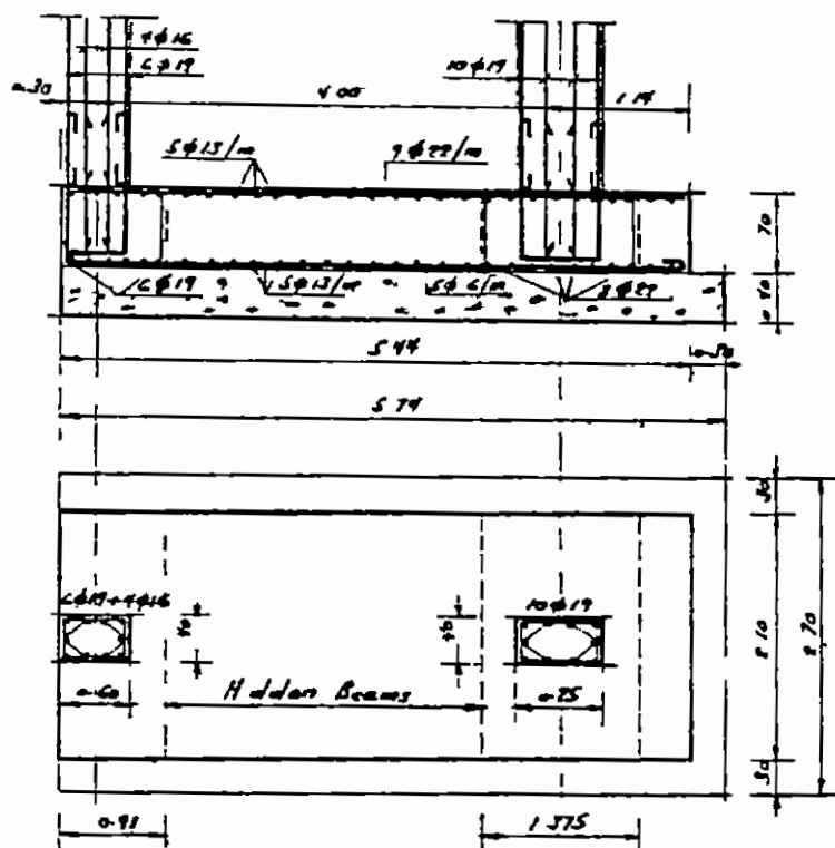
DETAILS OF A COMBINED FOOTING
