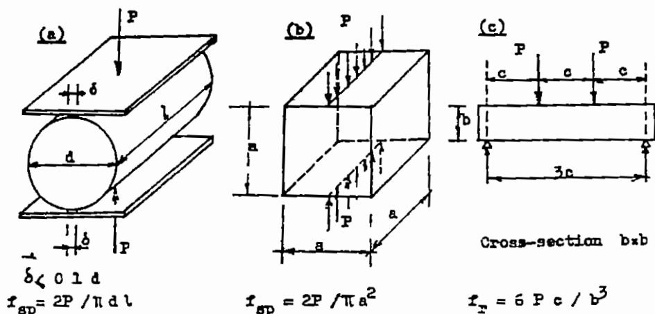
Fig 1-22 Types of specimens for tensile strength of concrete
