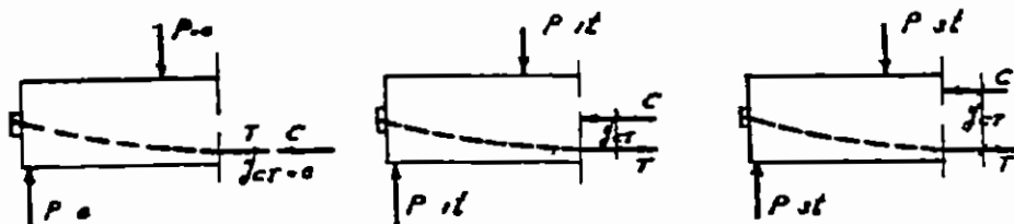
b) Variation of j_{cr} in a Prestressed Beam
