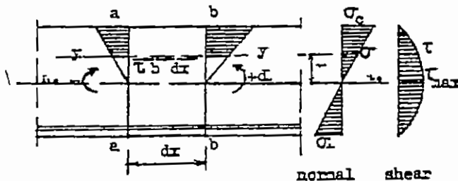
Fig 2-30 Normal and shear stresses in non- cracked linear stage
