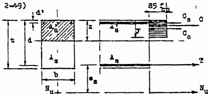
Fig 2-49 Ultimate stresses in a rectangular section subject to eccentric tension with big eccentricity
