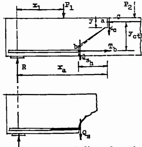
Fig 2-35 Forces at diagonal crack in beam without web reinforcement
