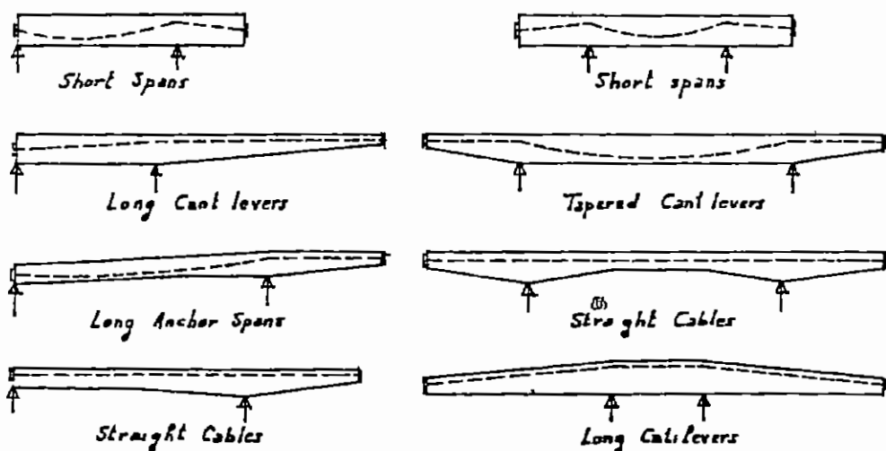
TYPICAL LAYOUTS FOR SINGLE CANTILEVERS DOUBLE CANTILEVERS
