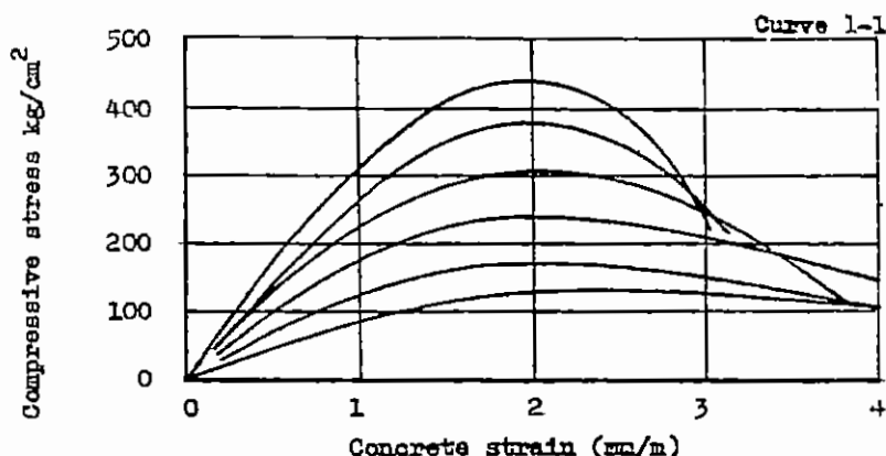
Fig. 1-21 Typical stress-strain curves at an age of 28 days from compression tests on concrete prisms
