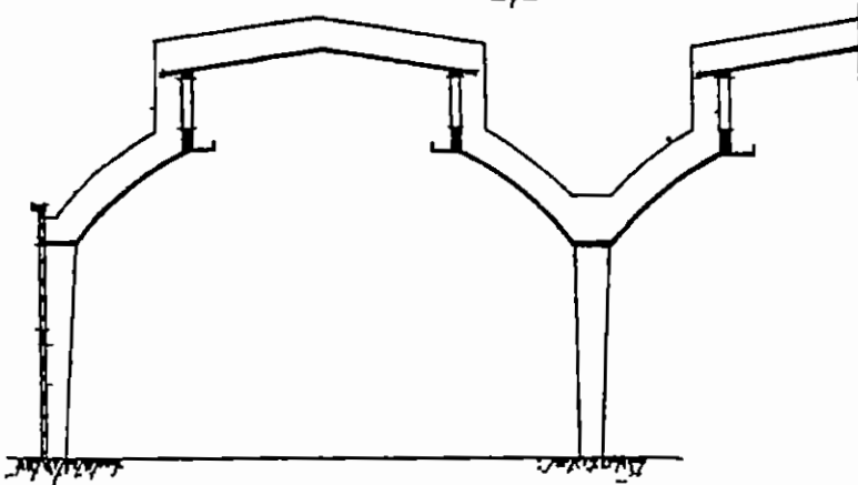
Fig 1-7 A 3-bay Hall in a Factory covered by Rigid Cont. Frames
