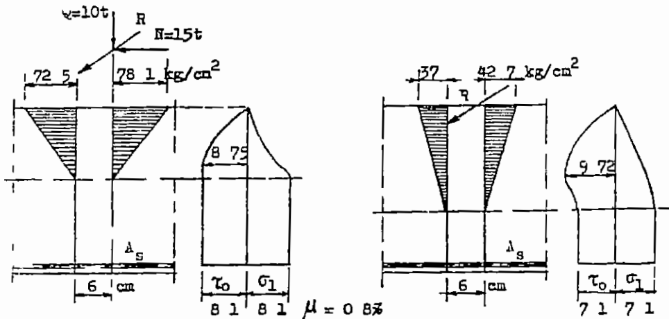
Fig 2-51 Shear and principal tensile stresses in sections subject to eccentric forces with big eccentricity
