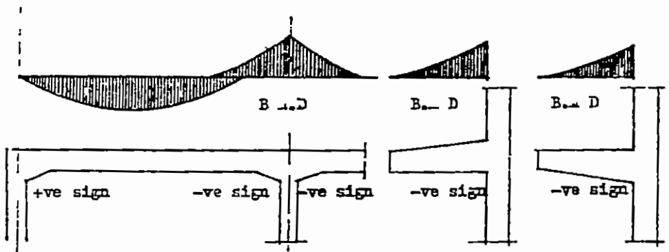
Fig 2-34 Sign of reduced shearing force
