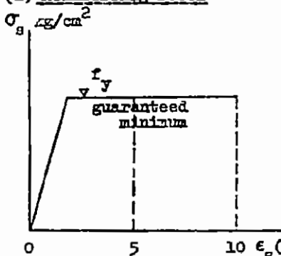
Fig. 2-20a Stress-strain relation-ship according to CEB
