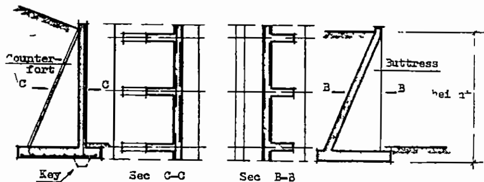
d- Counterforted wall
