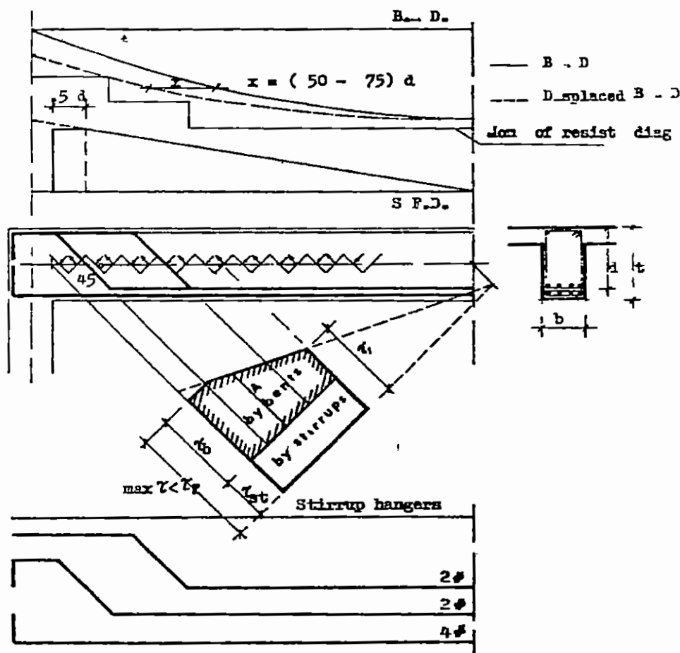
Fig 4-30 Determination of web reinforcement
