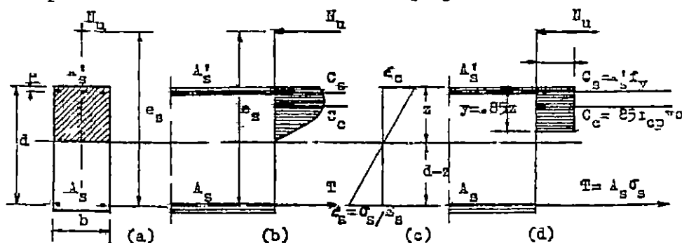
Fig. 2-45 Ultimate stresses in a rectangular section subject to eccentric compression
