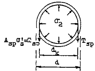
Fig 2-2 Resistance of spirals
