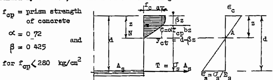
Fig 2-22 Distribution of stresses and strains at failure
