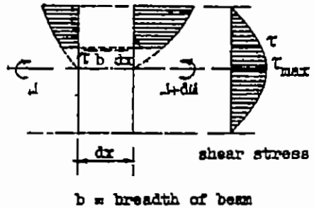
Fig 2-8 Shear stress distribution in a homogeneous beam
