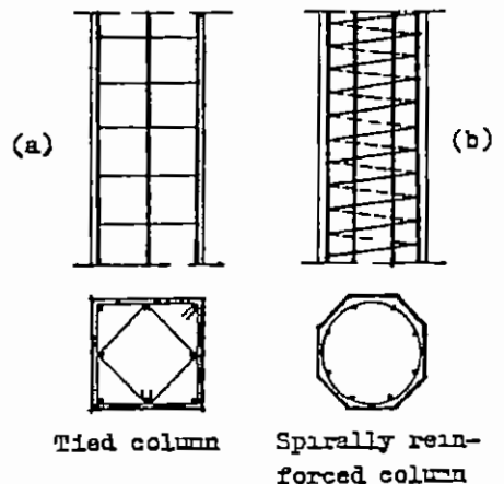
Fig 2-1 Chief forms of columns
