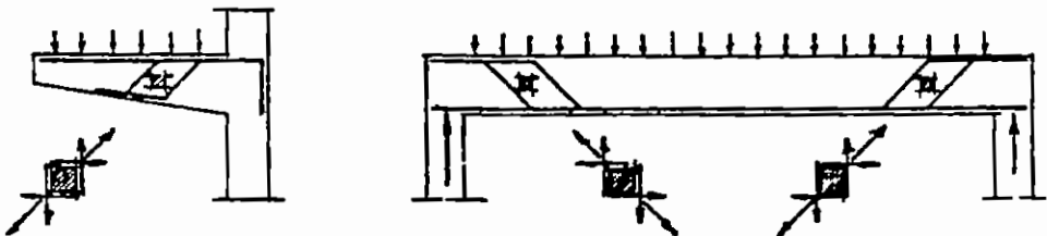
Fig 2-32 Determination of direction of diagonal tension
