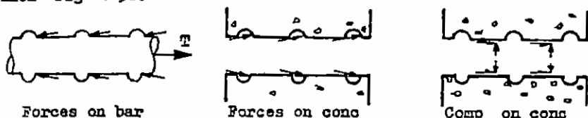
Flexural bond and anchorage bond
