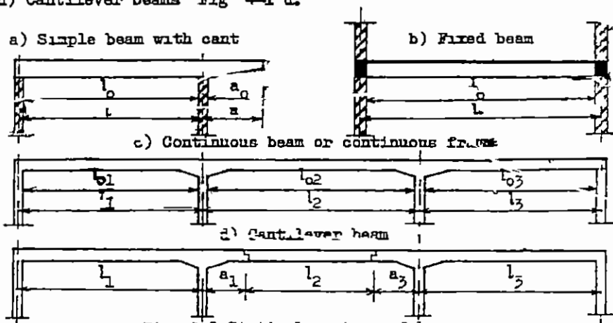
Fig. 4-1 Statical systems of beams
