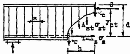
Fig 2-37 Forces at diagonal crack in beam with vert stir
