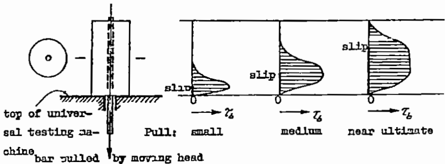
Fig 4-42: Pullout test and bond stress distribution
