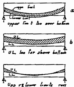
Undesirable positions for c.g.s. zone limits
