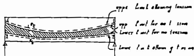
Limiting zone for c.g.s. allowing tension in concrete
