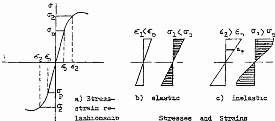
Fig. 2-7 Elastic and inelastic stress distribution in a homogeneous beam
