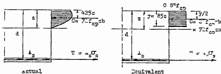
Fig 2-22' Stress-distribution at ultimate load (for f_{cp} < 280 \text{ kg/cm}^2 )
