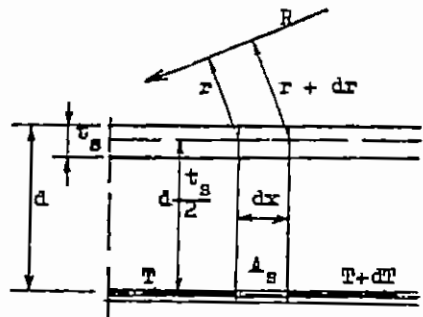
Fig 2-52 Shear in T-sections subject to eccentric forces
