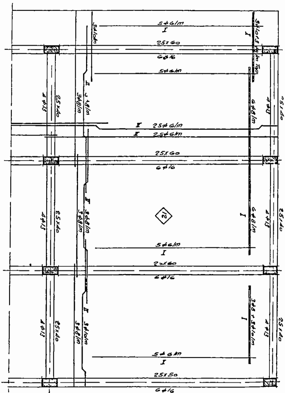
Fig 5-8 Example of a one-way slab
