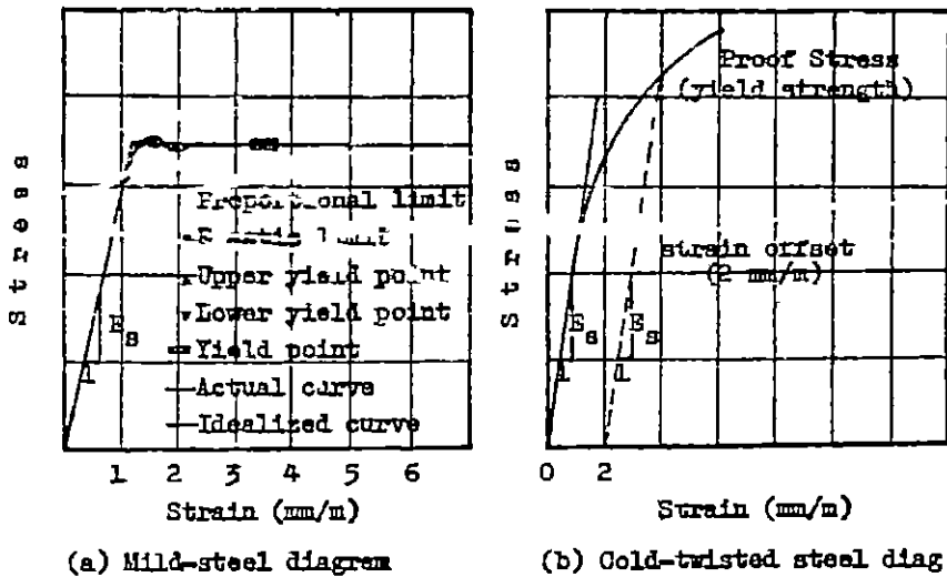
Fig 1-26 Stress-strain diagrams identification of yield point and yield strength
