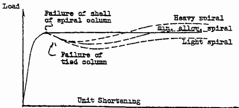
Fig 2-6 Comparison of strains in tied & spiral columns
