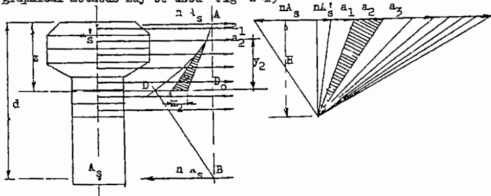
Fig 2-19 Graphical determination of stresses
