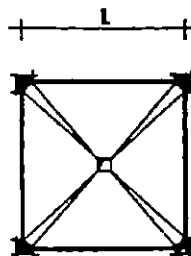
Fig 1-19 A Bunker
