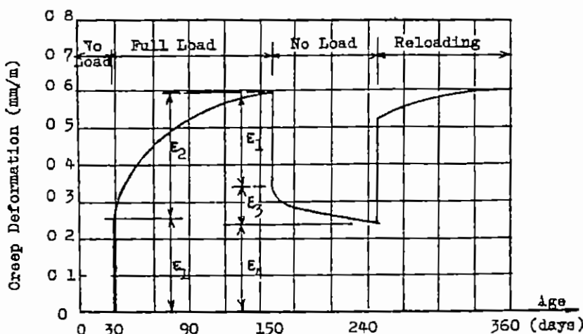
Fig 1-23 Creep deformations Influence of age and loading sequence
