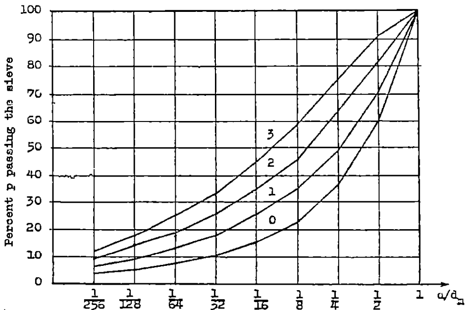
Fig. 1-21 Grading curve of aggregates
