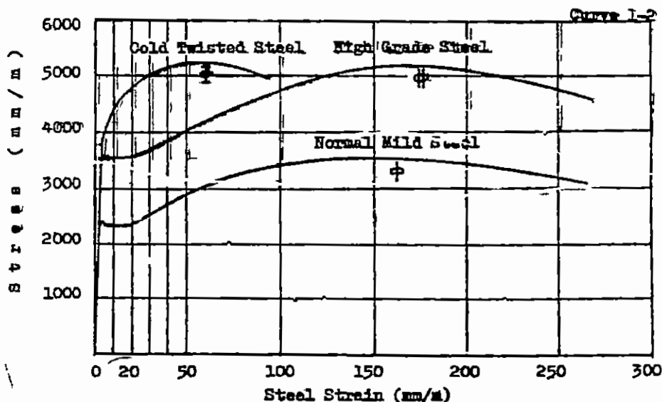
Fig 1-25 Typical stress-strain curves for reinforcing bars of different steel characteristics
