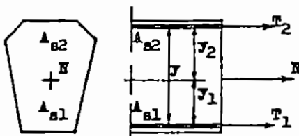
Fig 2-47 Eccentric tension with small eccentricity
