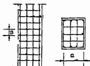
Fig 2-3 Cross-reinforced member
