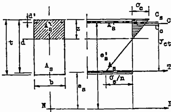
Fig. 2-48 Stresses in a rectangular section subject to eccentric tension with big eccentricity
