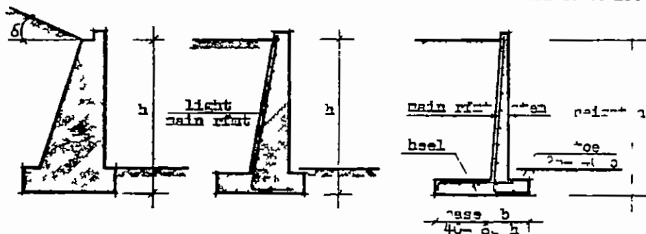
a- Gravity wall
