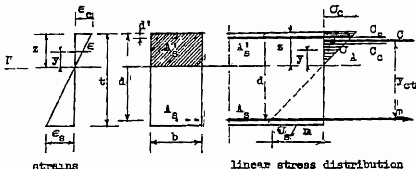
Fig 2-10 Linear stress distribution in a reinforced concrete rectangular section subject to simple bending
