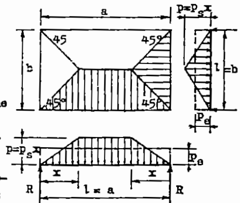
Fig 4-3 Load on beams supporting two-way slabs with similar edge conditions
