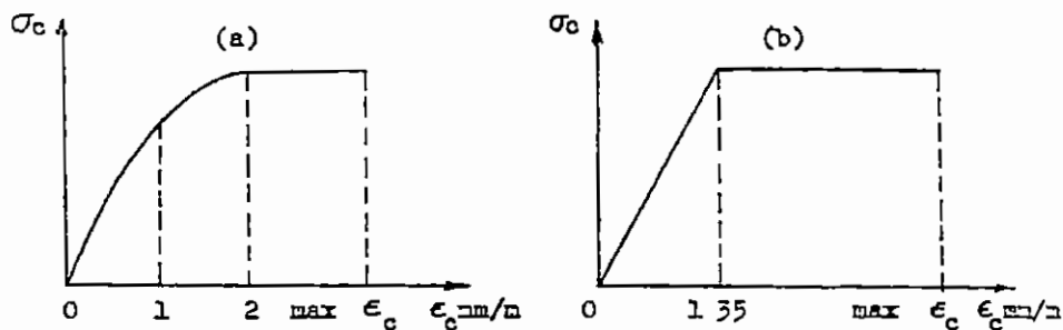
Fig 2-21 Idealized concrete stress-strain relationship
