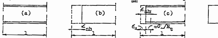
Fig 2-4 Evaluation of shrinkage stresses
