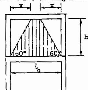
Fig 4-6 Wall load
