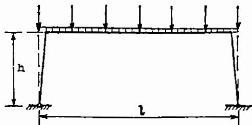
Fig 3.6 Main frames
