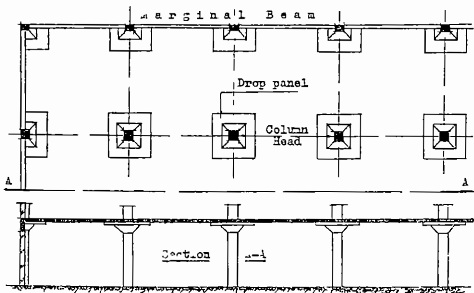
Fig 1-3 A Flat-slab
