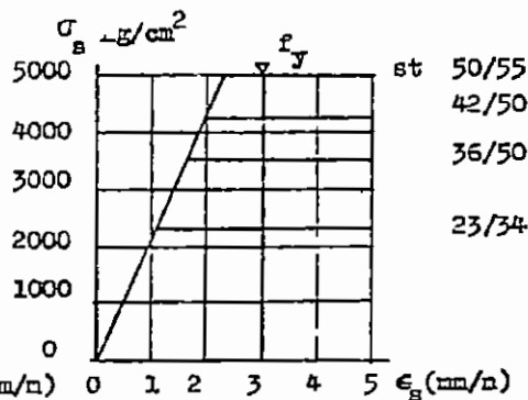
Fig. 2-20b Stress-strain relationship according to DIN
