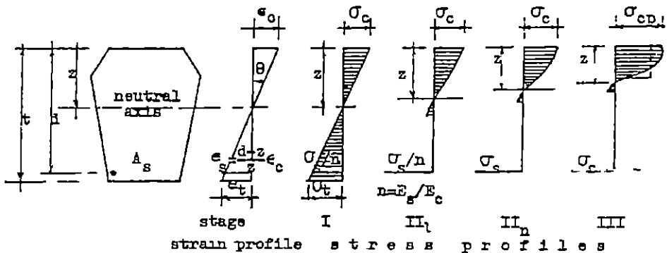
Fig 2-9 Distribution of strains and stresses for various stages of loading
