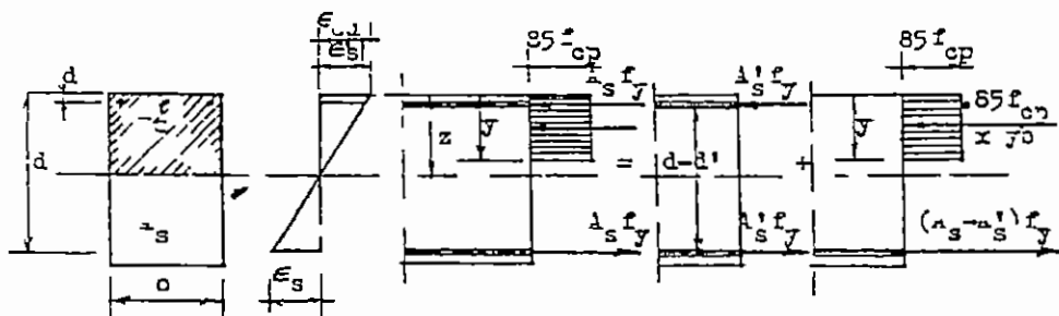
Fig 2-25 Rectangular section with double reinforcement
