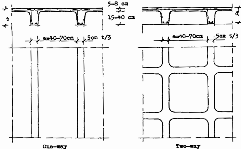
Fig 5-12 Ribbed slabs
