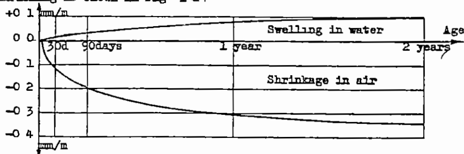
Fig. 1-24 Shrinkage in air and swelling in water during hardening
