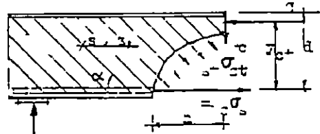
Fig 2-38 Forces at diag crack in beam with inclined web rivet
