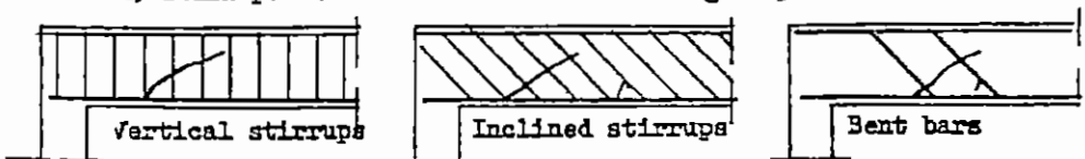
Fig 2-36 Web reinforcements of reinforced concrete beams
