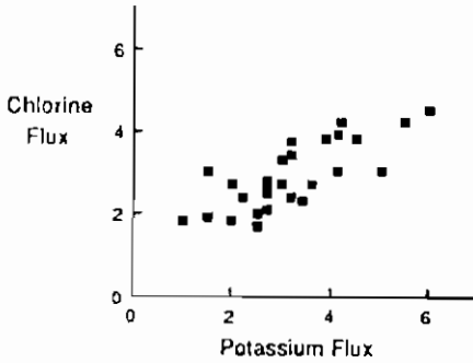
SCATTERGRAM
