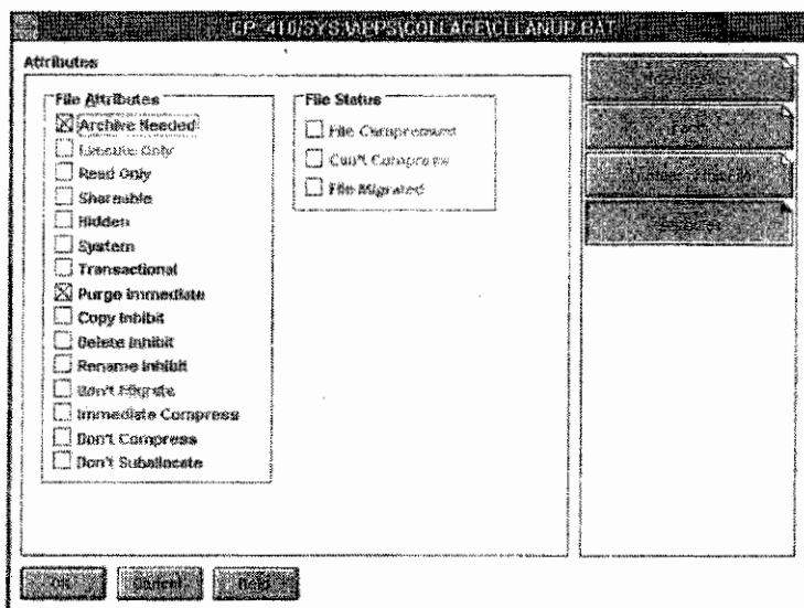
The CLEANUP.BAT File Attribute page, with Purge Immediate marked.
